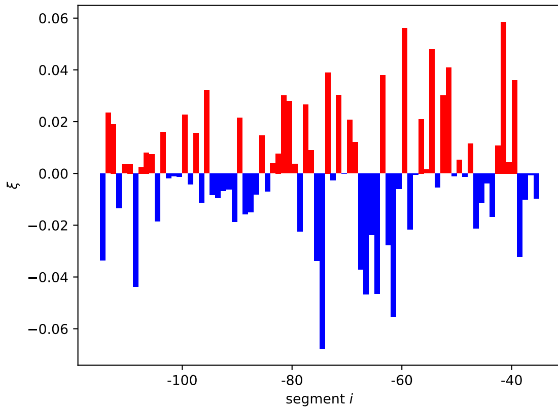
cra expression shift \xi_i[01, 10]
