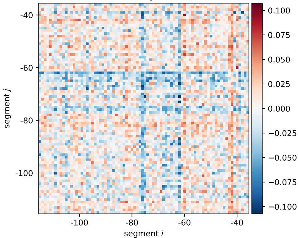
cra expression shift \xi_{i,j}[0101, 0110, 1010]
