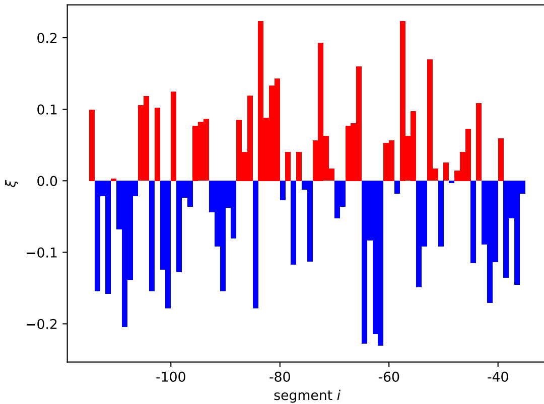
cra expression shift \xi_i[01, 10]
