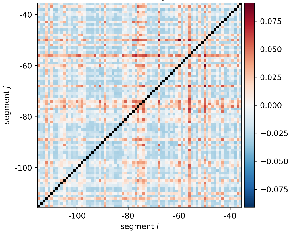
dicA expression shift \xi_{i,j}[0011, 1100]
