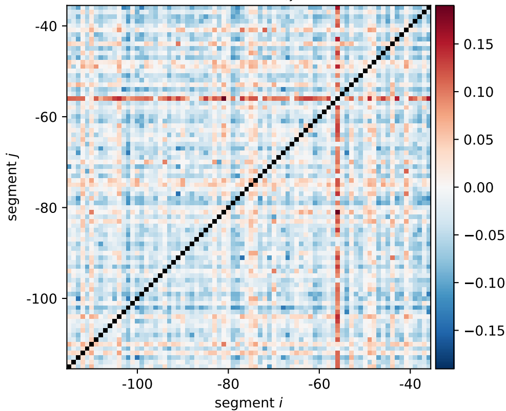
dicA expression shift \xi_{i,j}[0011, 1100]
