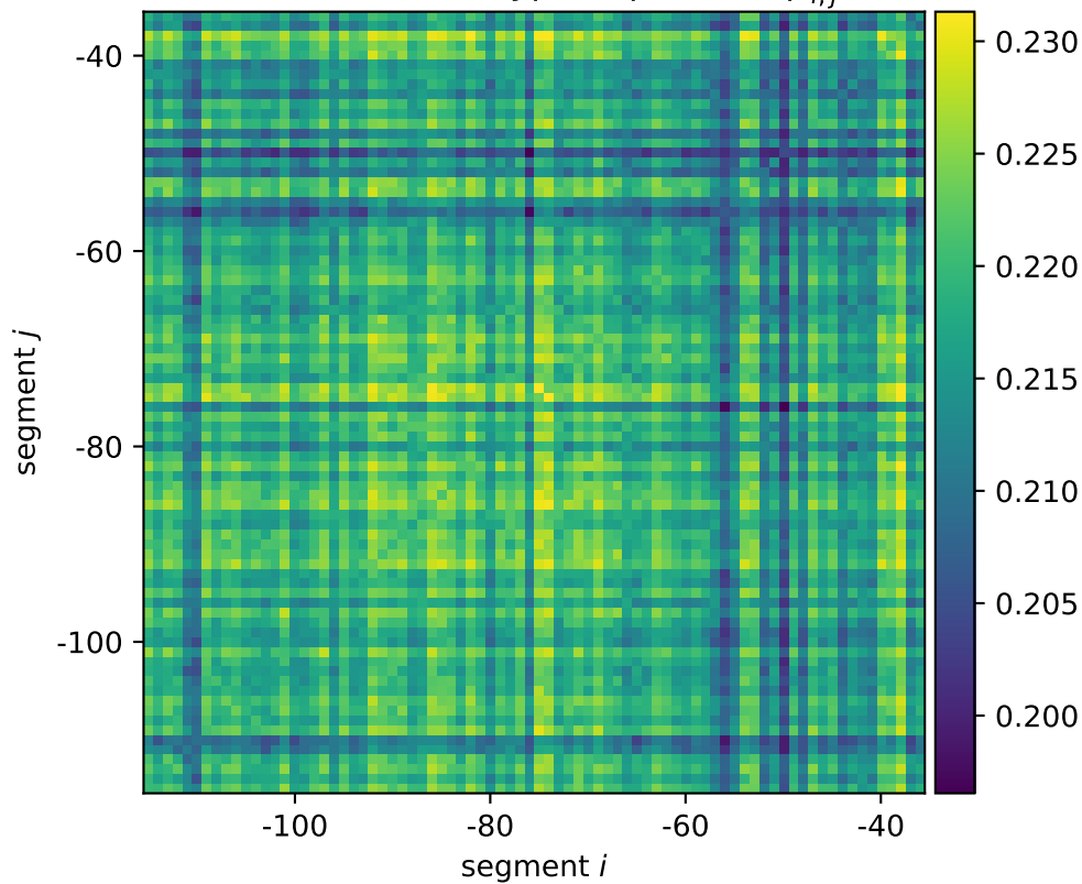
dicA mean wildtype expression \mu_{i,j}^*
