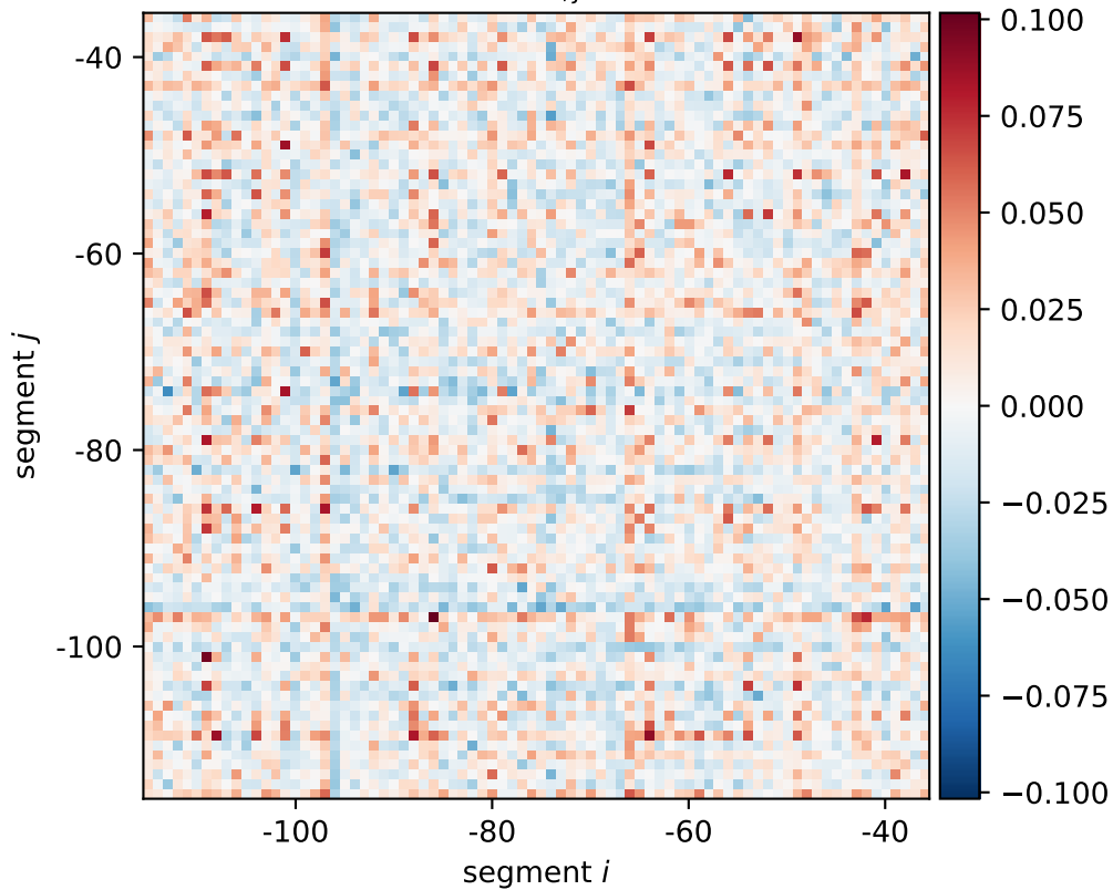
dicB expression shift \xi_{i,j}[0101, 0110, 1010]
