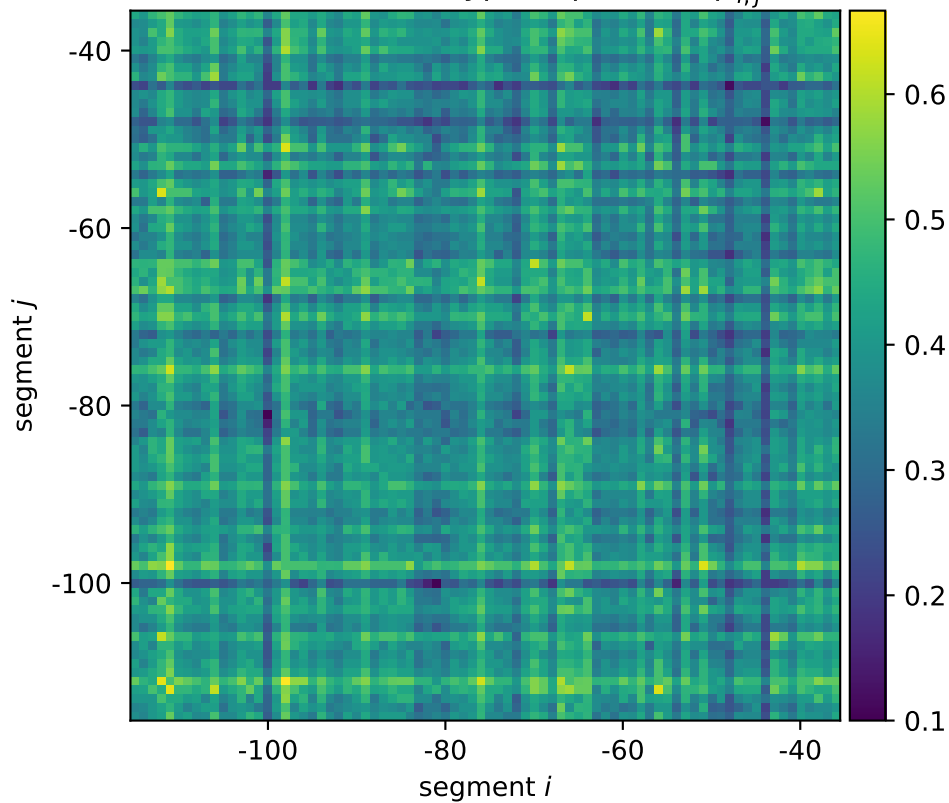
dicB mean wildtype expression \mu_{i,j}^*
