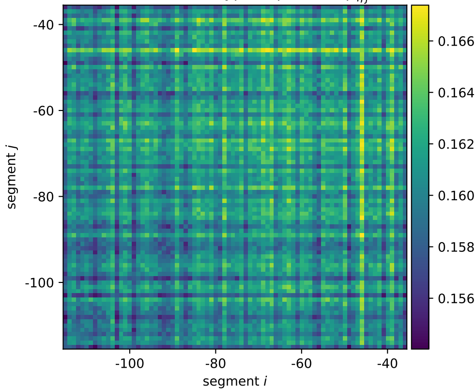
dicB mean wildtype expression \mu_{i,j}^*
