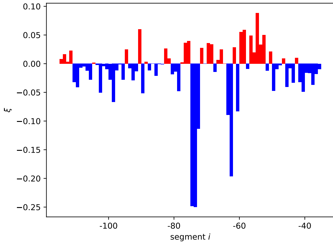
dicC expression shift \xi_i[01, 10]
