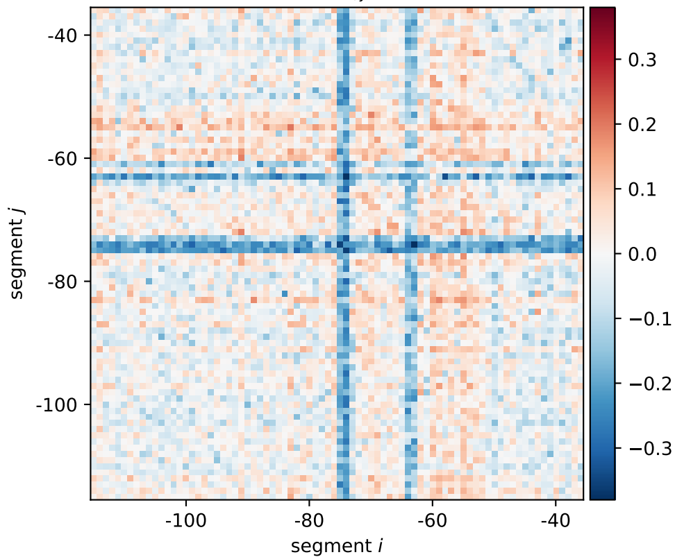
dicC expression shift \xi_{i,j}[0101, 0110, 1010]
