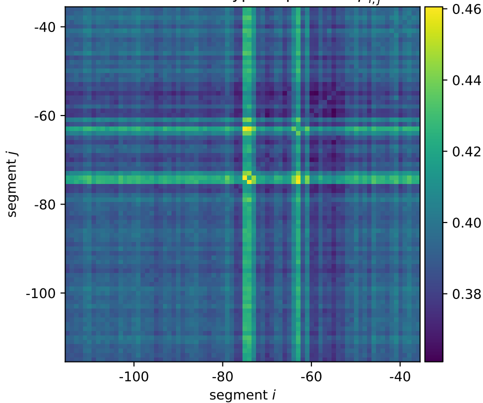
dicC mean wildtype expression \mu_{i,j}^*
