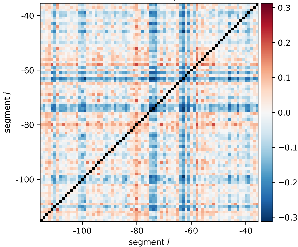
dicC expression shift \xi_{i,j}[0011, 1100]
