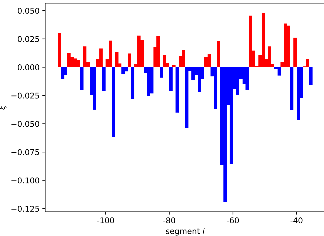
dinJ expression shift \xi_i[01, 10]
