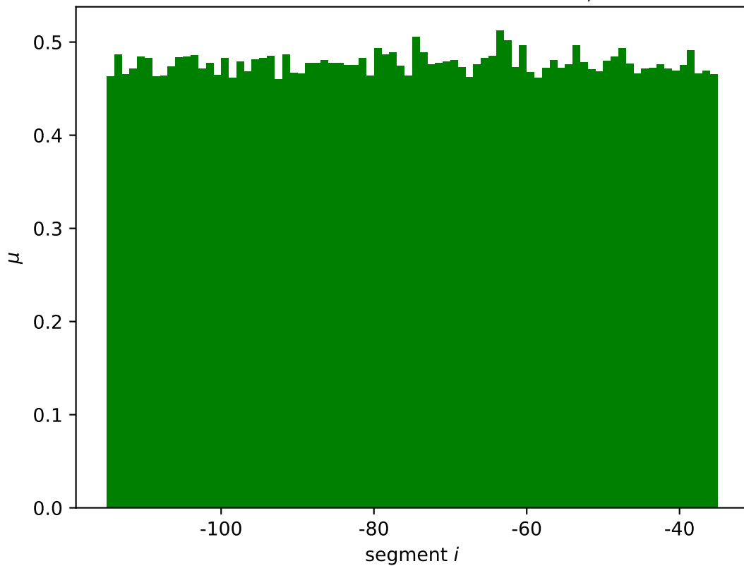
dinJ mean wildtype expression \mu_i^*
