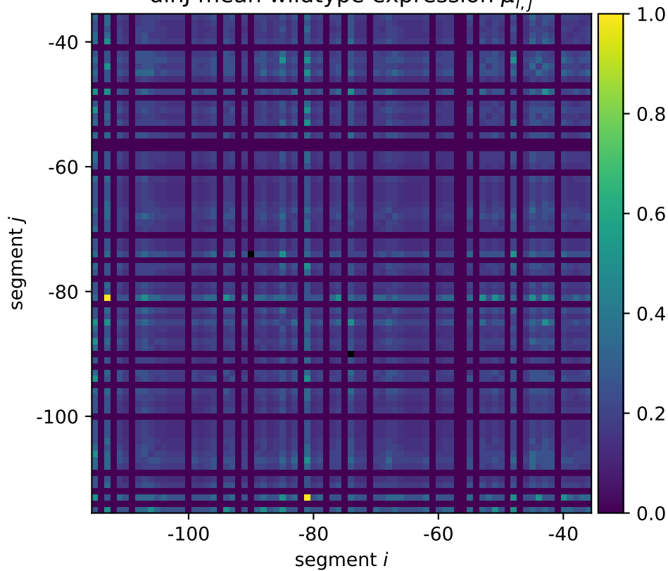
dinJ mean wildtype expression \mu_{i,j}^*
