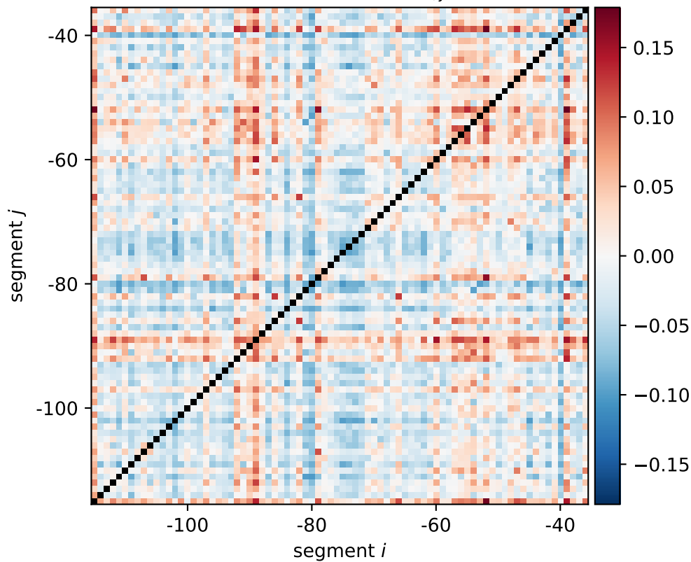
dnaE_start1 expression shift \xi_{i,j}[0011, 1100]
