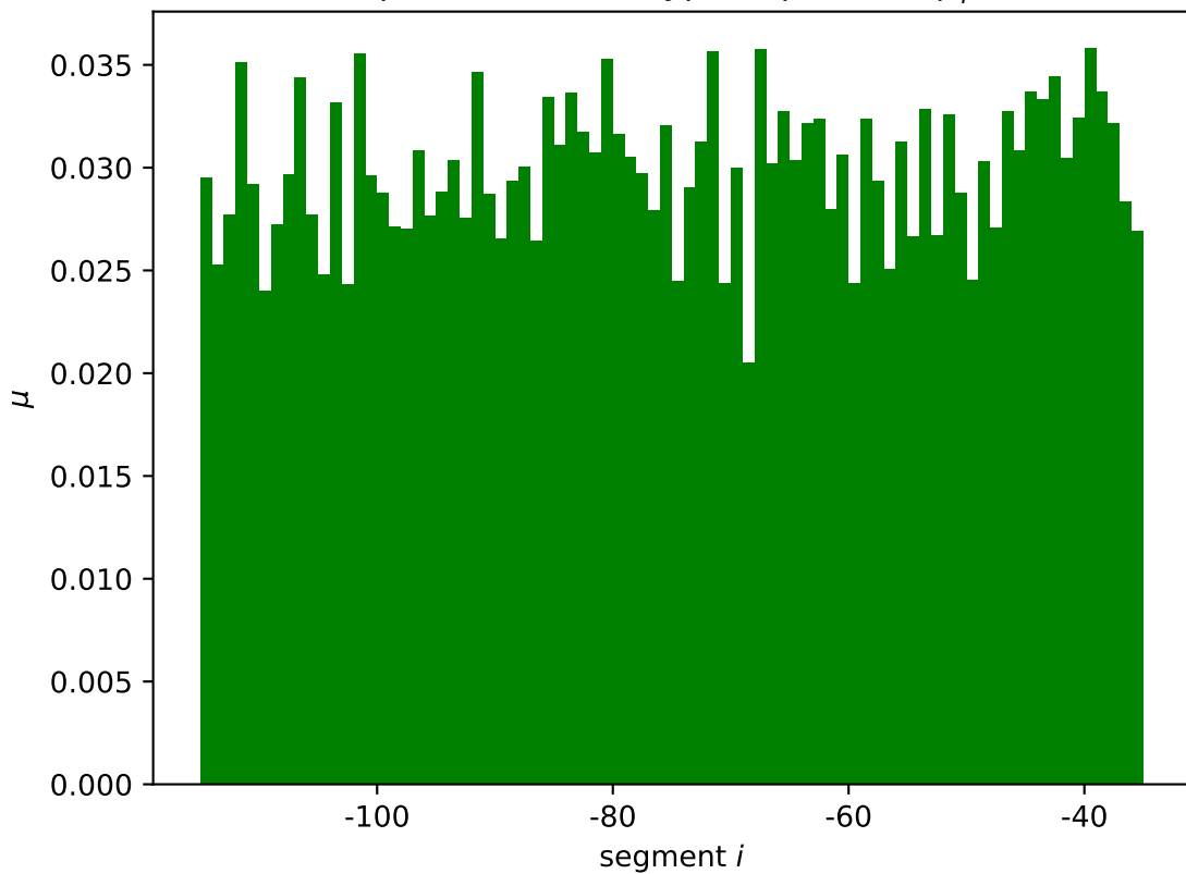
dpiBA mean wildtype expression \mu_i^*
