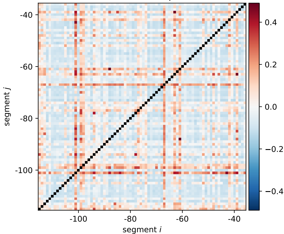
dpBA expression shift \xi_{i,j}[0011, 1100]
