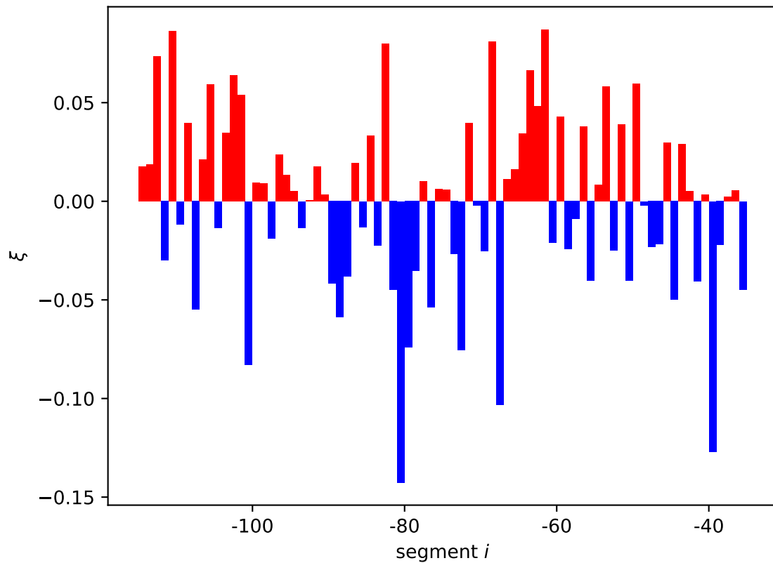
dpiBA expression shift \xi_i[01, 10]
