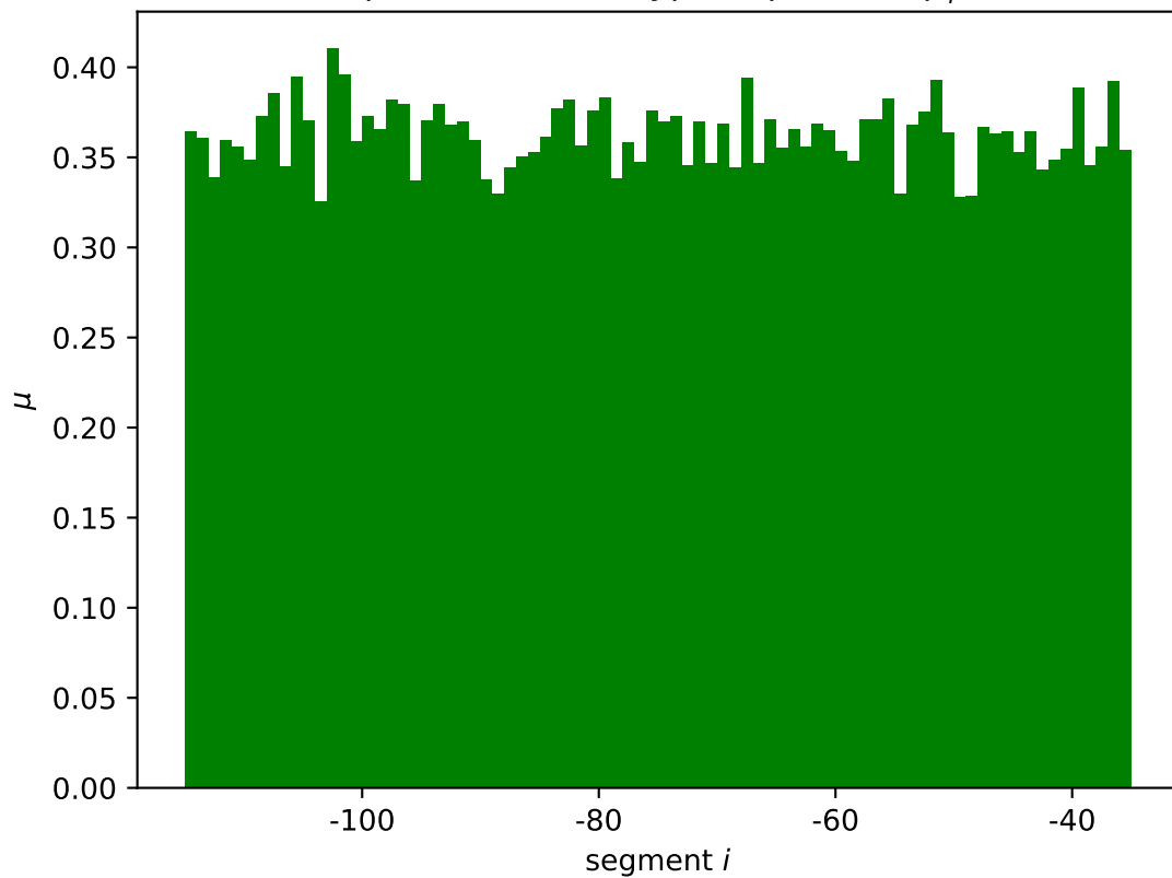
dpiBA mean wildtype expression \mu_i^*
