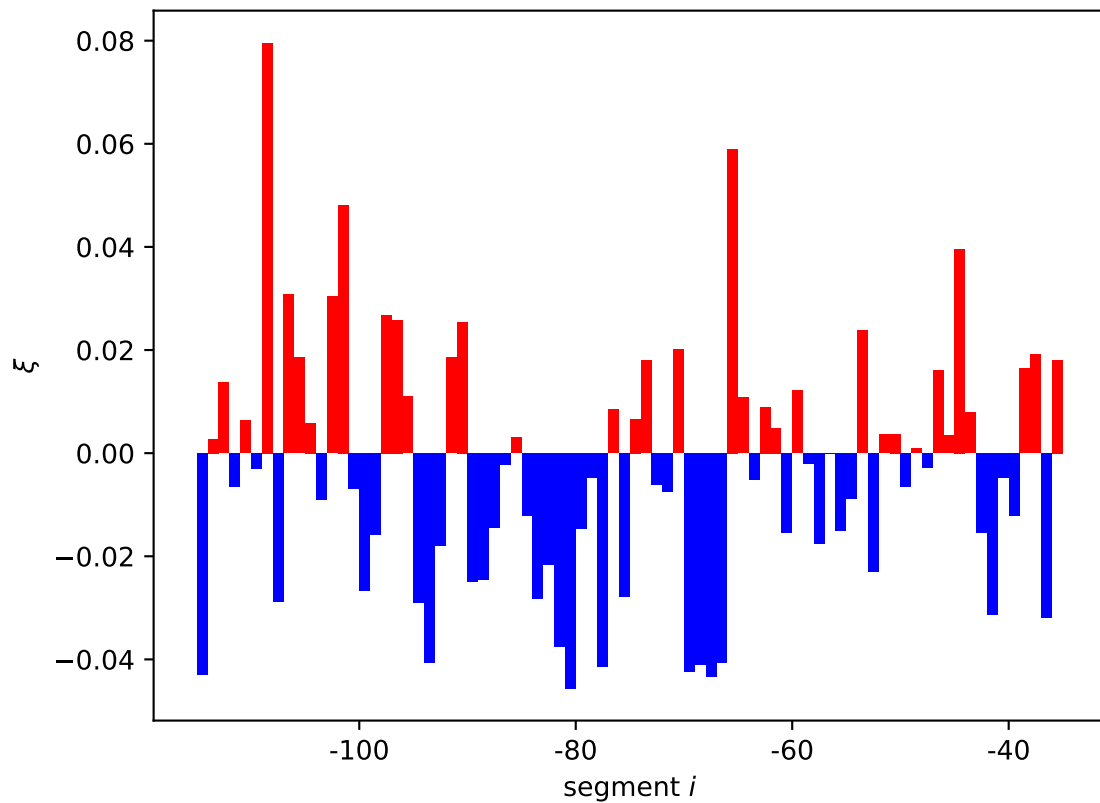
duSC expression shift \xi_i[11]
