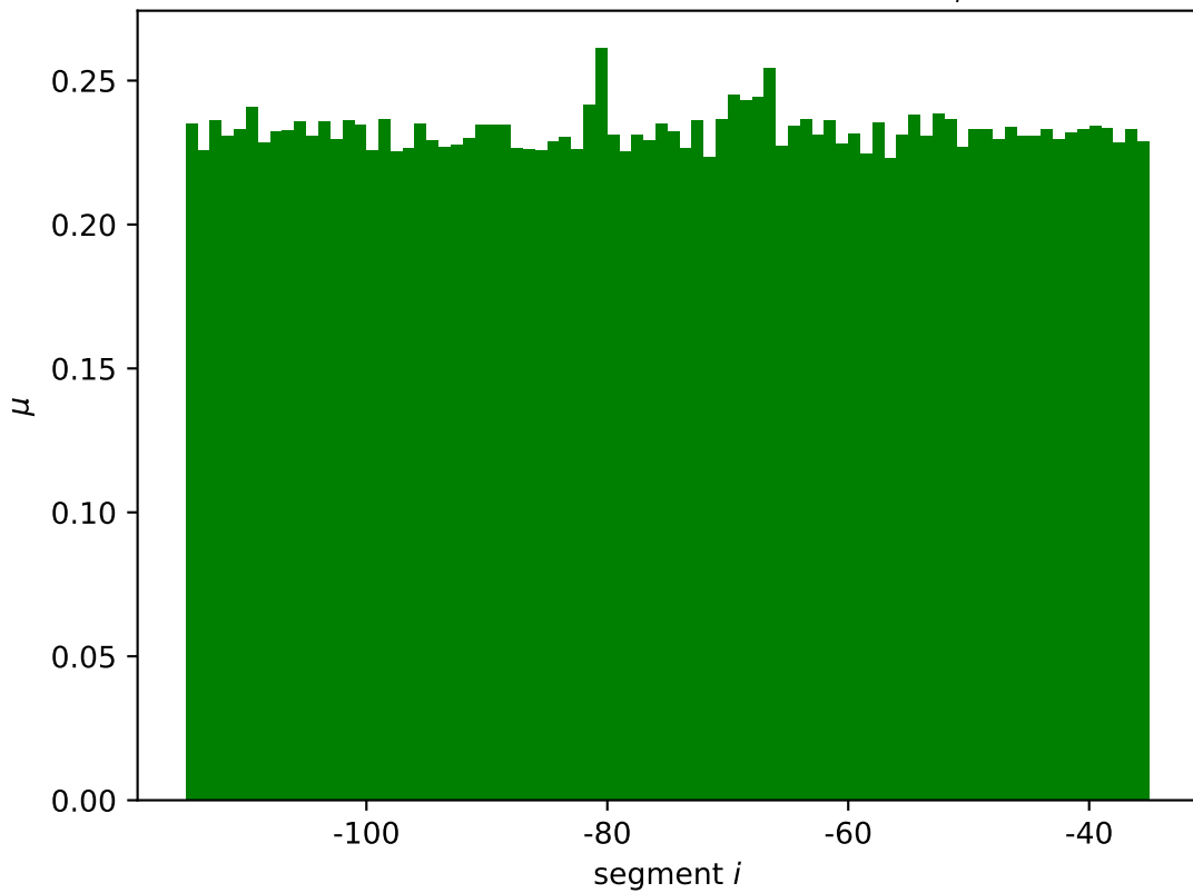
duxC mean wildtype expression \mu_i^*
