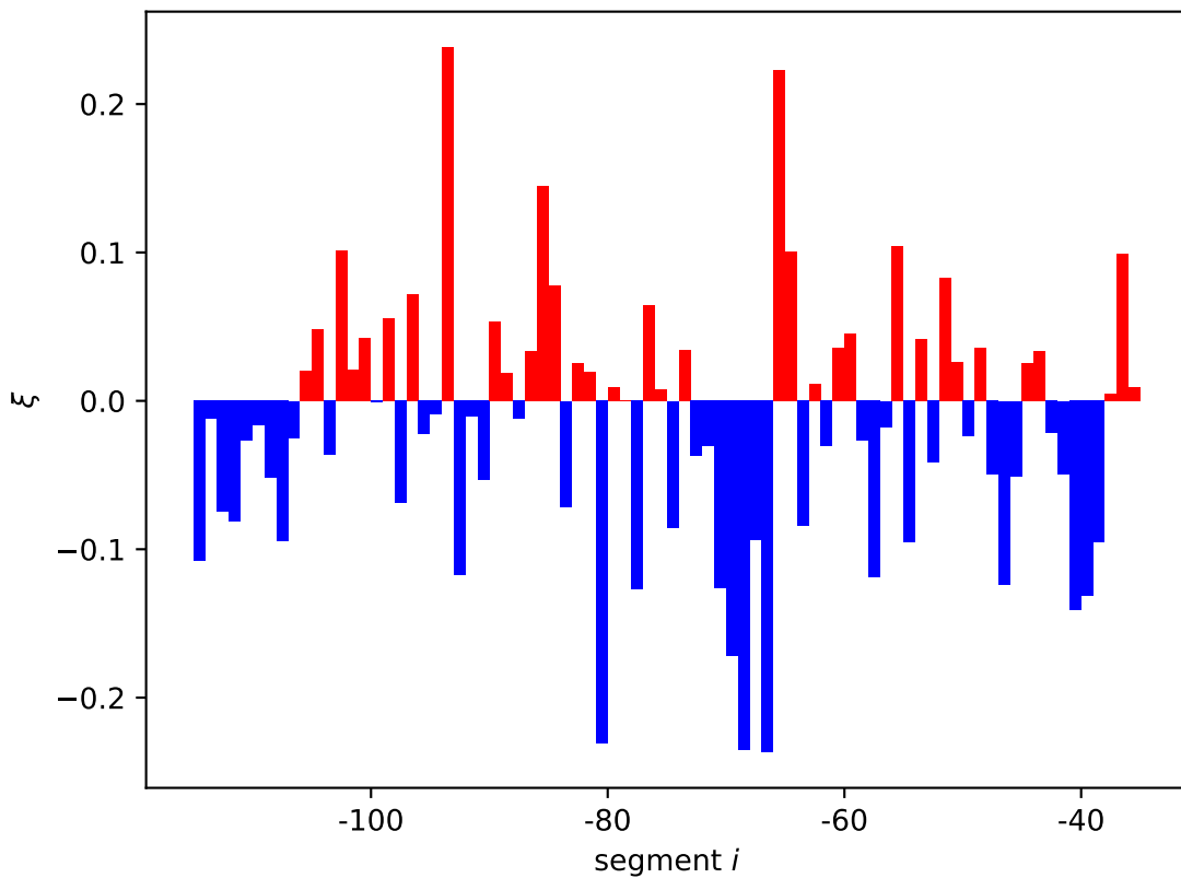
duSC expression shift \xi_i[11]
