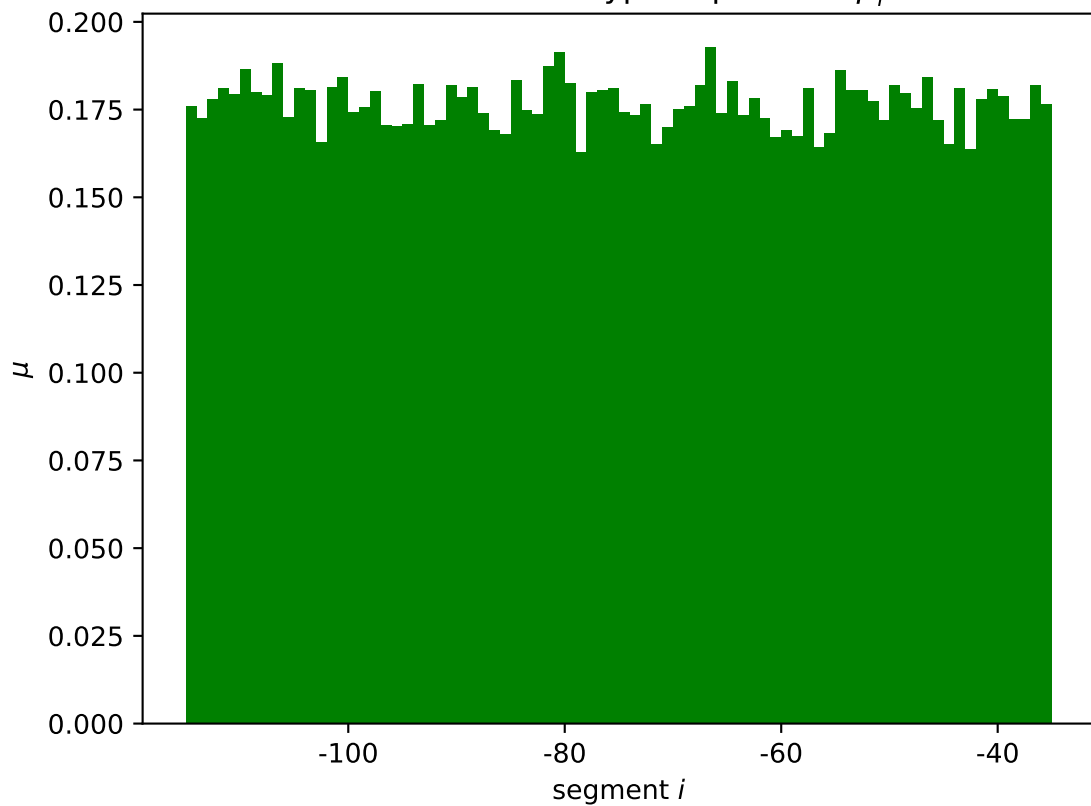
duxC mean wildtype expression \mu_i^*
