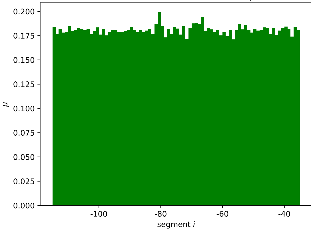
duoC mean wildtype expression \mu_i^*
