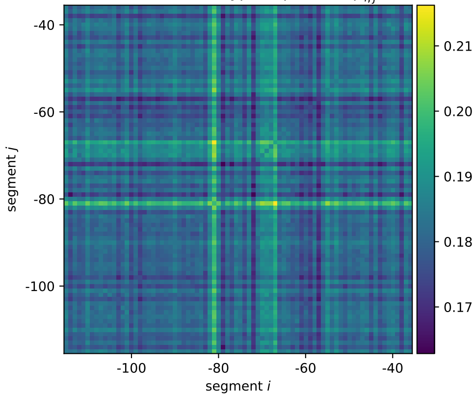
duC mean wildtype expression \mu_{i,j}^*
