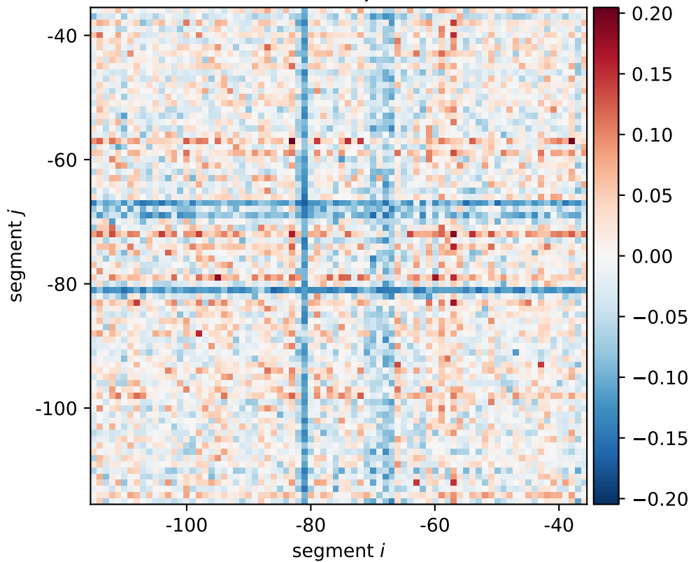
duC expression shift \xi_{i,j}[0101, 0110, 1010]
