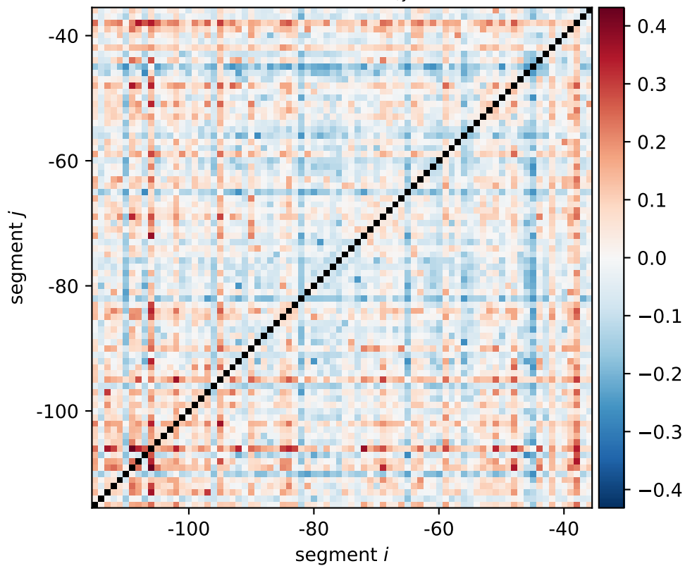
ecnB expression shift \xi_{i,j}[\text{0011}, \text{1100}]
