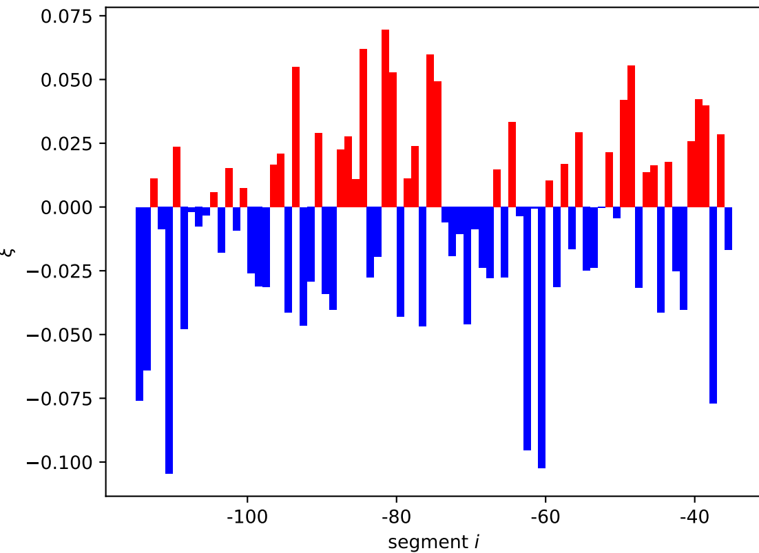
ecnB expression shift \xi_i[01, 10]
