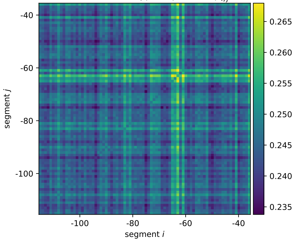
ecnB mean wildtype expression \mu_{i,j}^*
