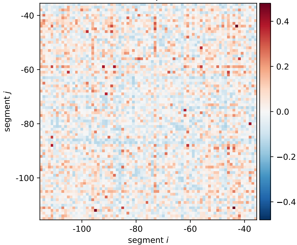
eco expression shift \xi_{i,j}[0101, 0110, 1010]
