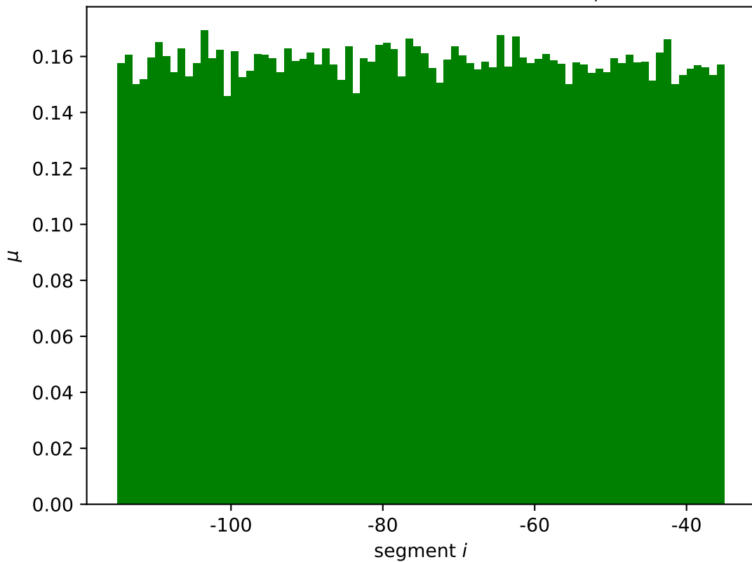
eco mean wildtype expression \mu_i^*
