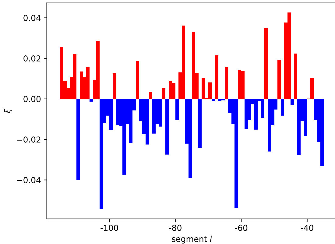
fdhE expression shift \xi_i[01, 10]
