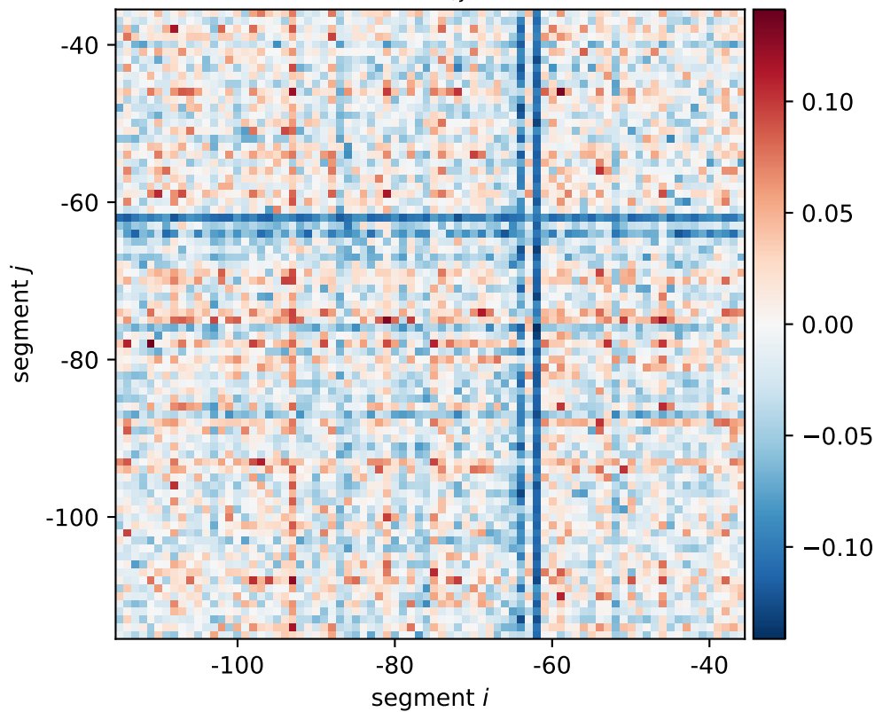
fdhE expression shift \xi_{i,j}[0101, 0110, 1010]
