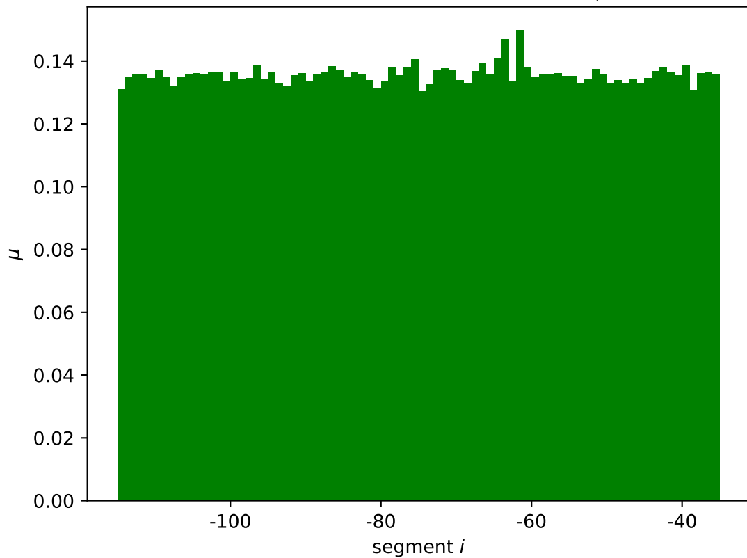
fdhE mean wildtype expression \mu_i^*
