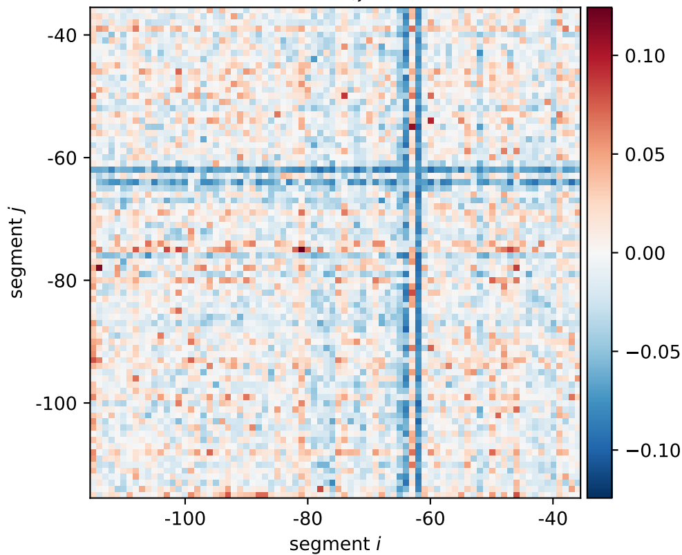
fdhE expression shift \xi_{i,j}[\text{0101}, \text{0110}, \text{1010}]
