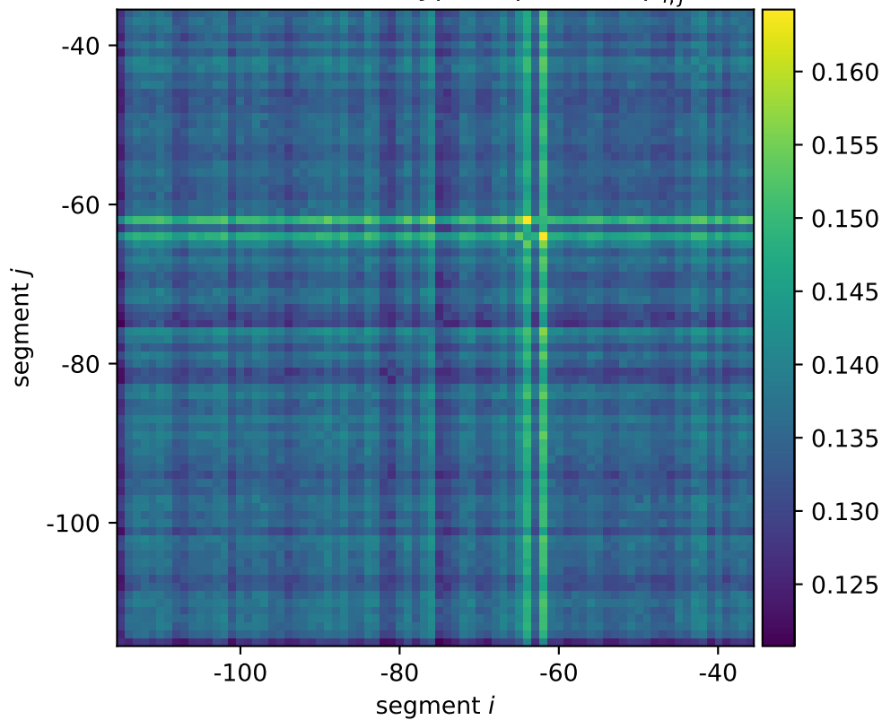
fdhE mean wildtype expression \mu_{i,j}^*
