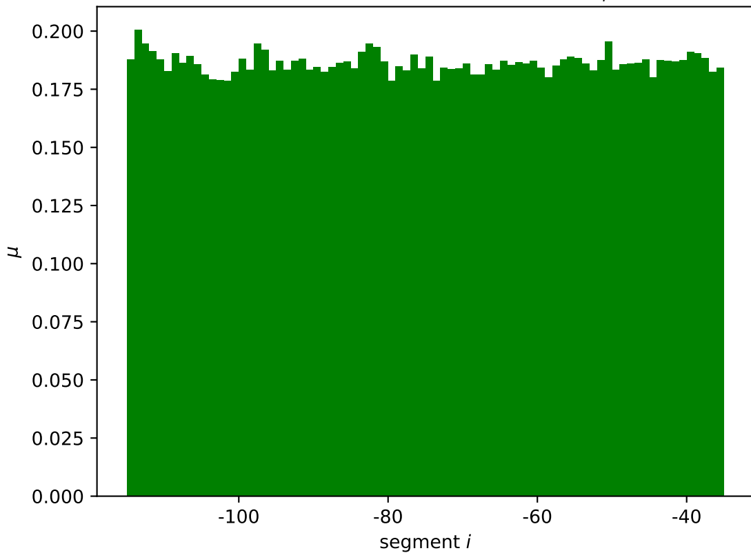
fdoH mean wildtype expression \mu_i^*
