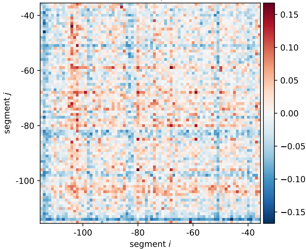
fdoH expression shift \xi_{i,j}[0101, 0110, 1010]
