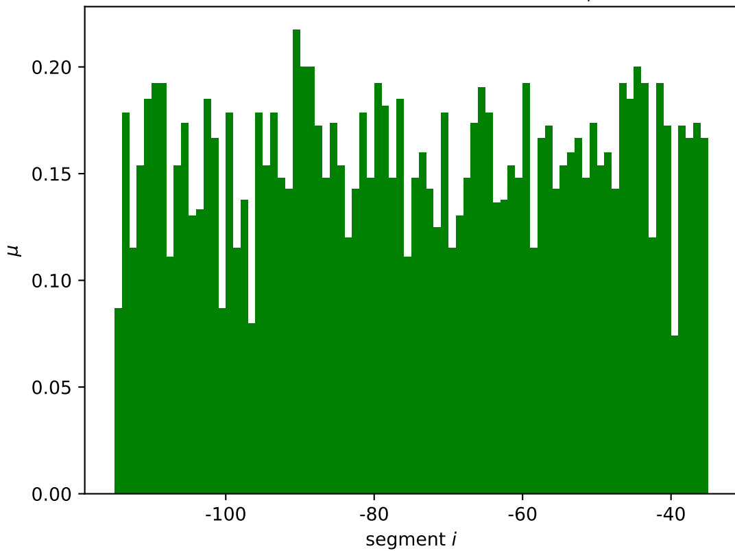
fdoH mean wildtype expression \mu_i^*
