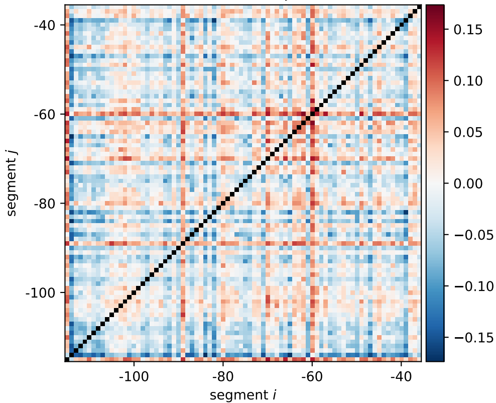
fdoH expression shift \xi_{i,j}[0011, 1100]
