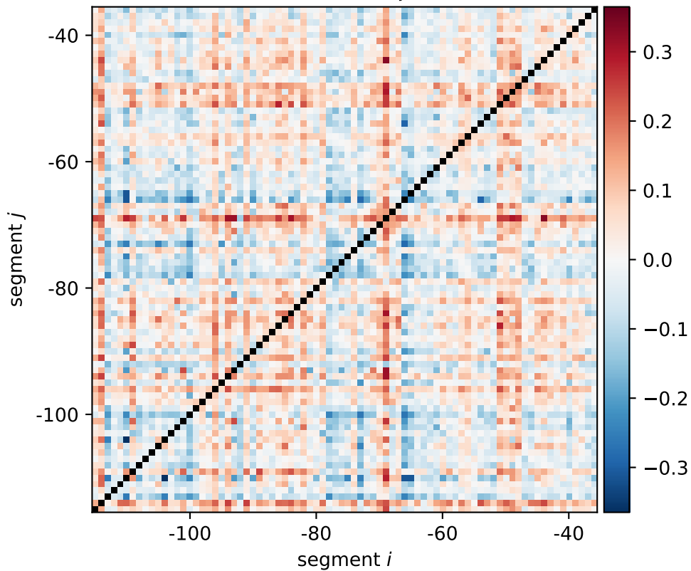
ftsK expression shift \xi_{i,j}[0011, 1100]
