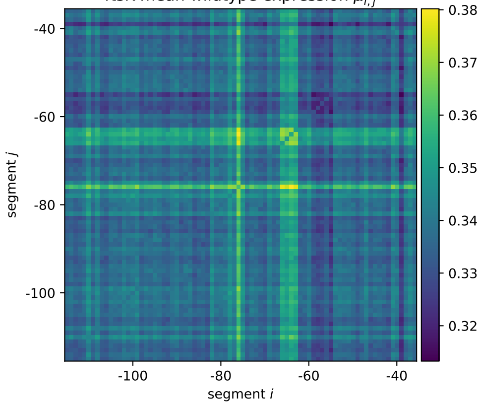
ftsK mean wildtype expression \mu_{i,j}^*
