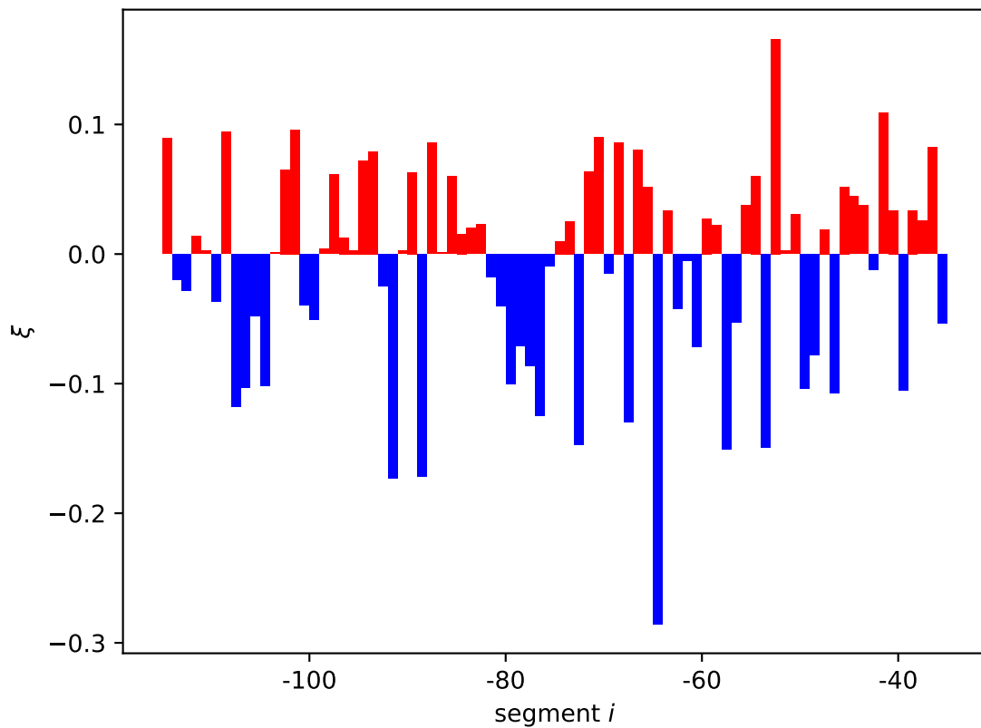
ftsK expression shift \xi_i[11]
