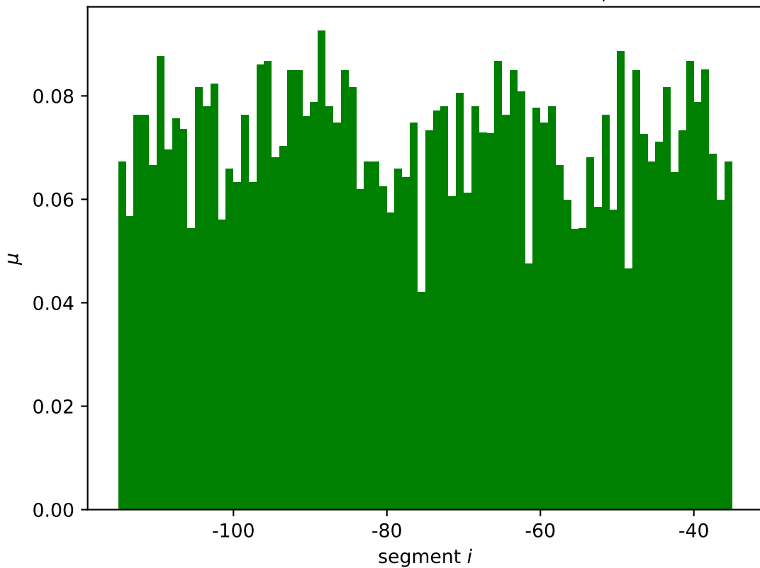
ftsK mean wildtype expression \mu_i^*
