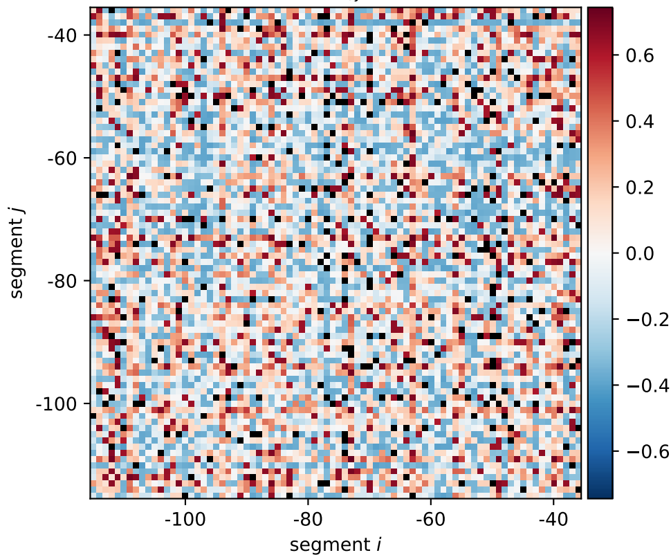
ftsK expression shift \xi_{i,j}[0101, 0110, 1010]
