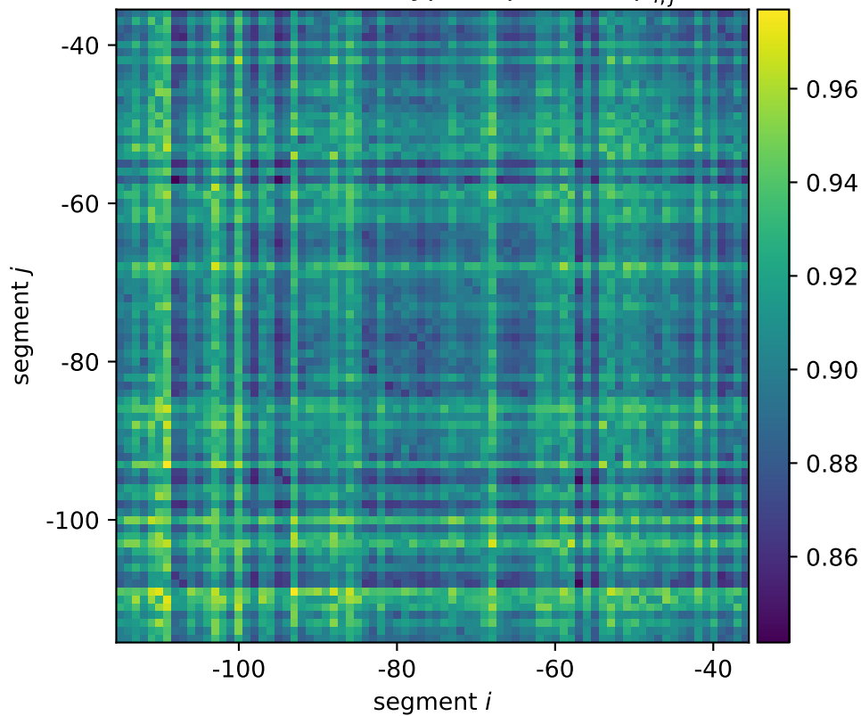
ftsK mean wildtype expression \mu_{i,j}^*
