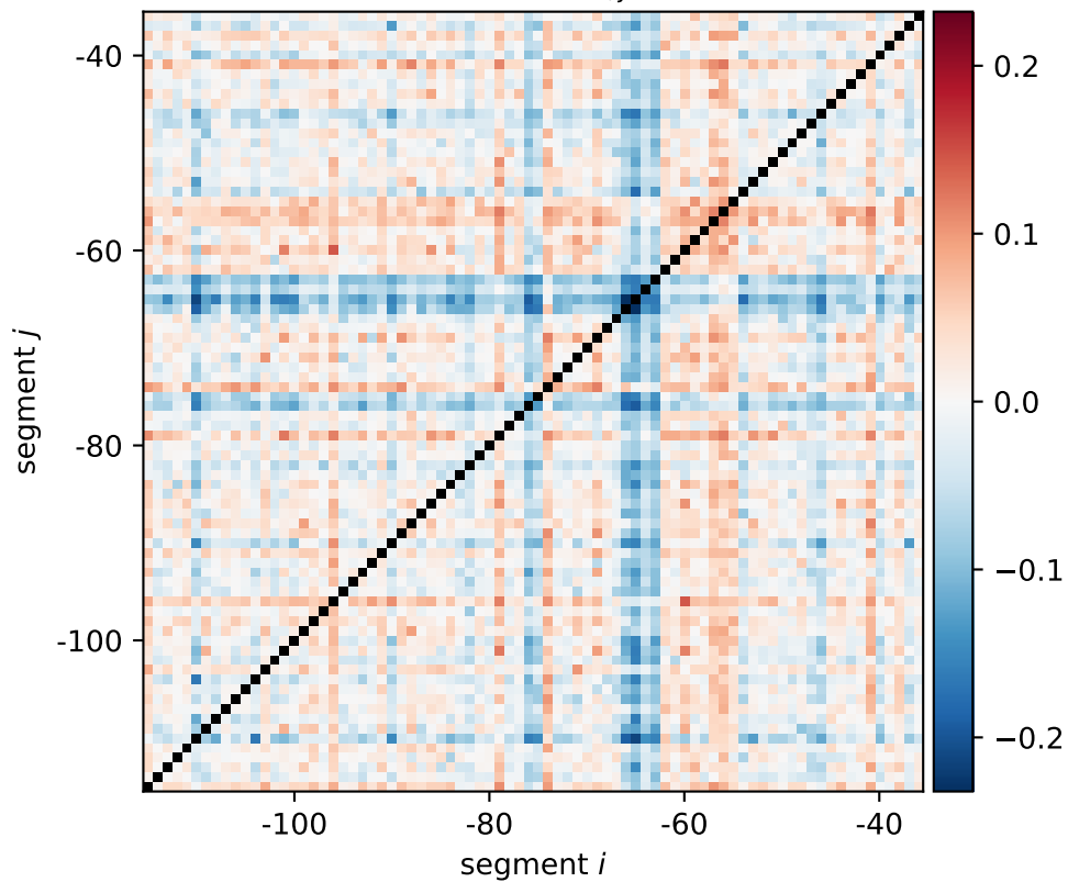
ftsK expression shift \xi_{i,j}[\text{0011}, \text{1100}]
