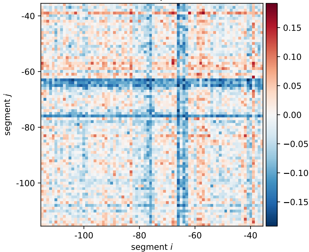
ftsK expression shift \xi_{i,j}[\text{0101}, \text{0110}, \text{1010}]
